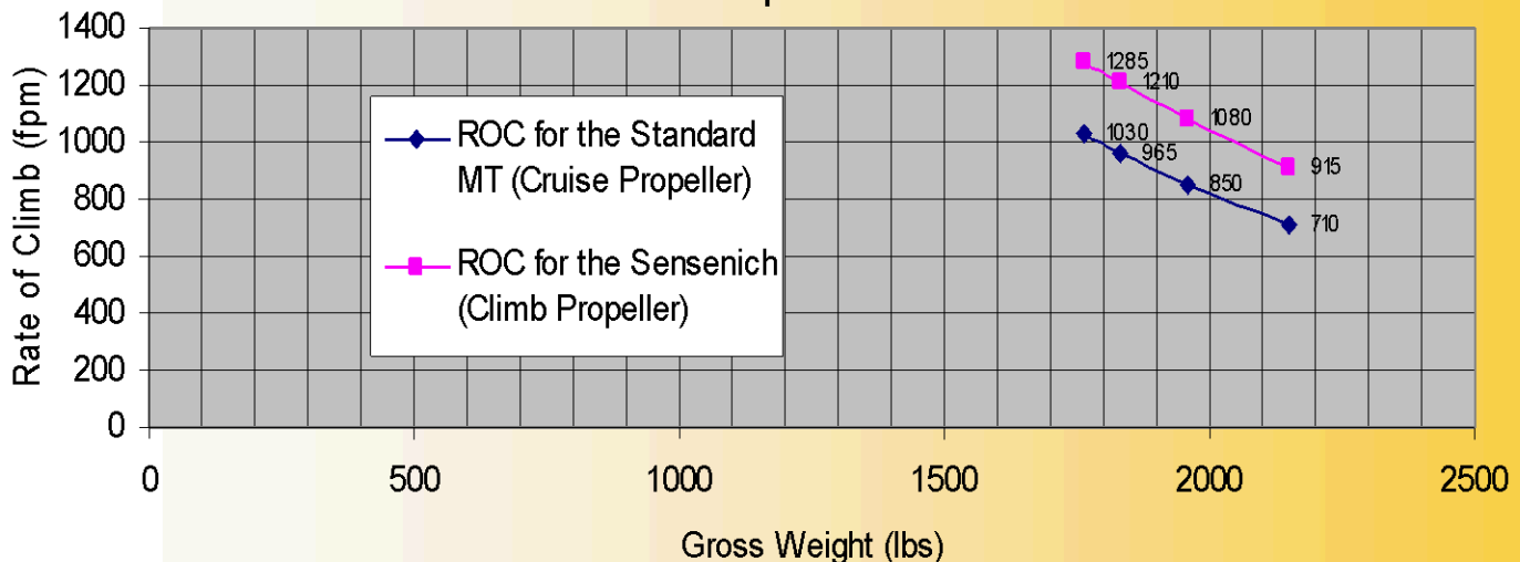
Sensenich & MT Propeller Standard Day (ISA) at Sea Level Comparison
